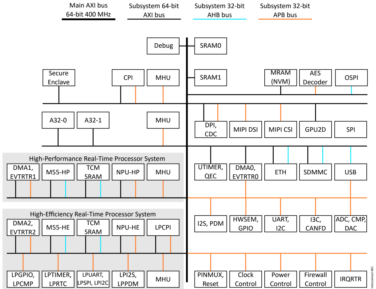
Figure 3-1 Interconnect Overview
